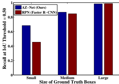
Figure 11. Comparison of recall of region proposals generated by AZ-Net and RPN for objects of different sizes on VOC 2007 test. The comparison is performed at \text{IoU} = 0.5 with top-300 proposals. Our approach has significantly better recall for small objects.
