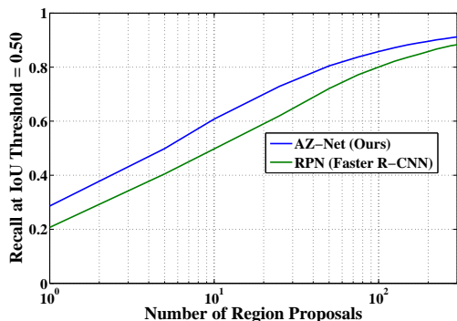
Figure 10. Comparison of recall of region proposals generated by AZ-Net and RPN at different number of region proposals on VOC 2007 test. The comparison is performed at \text{IoU} = 0.5 . Our approach has better early recall. In particular, it reaches 0.6 recall with only 10 proposals.
